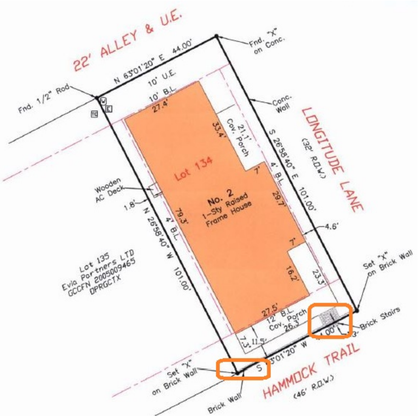
As-Built Survey Showing Encroachments
