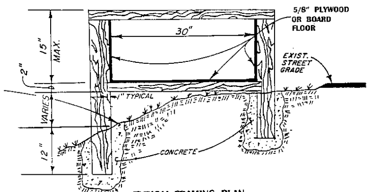
TYPICAL FRAMING PLAN FOR SLOPE AREAS
