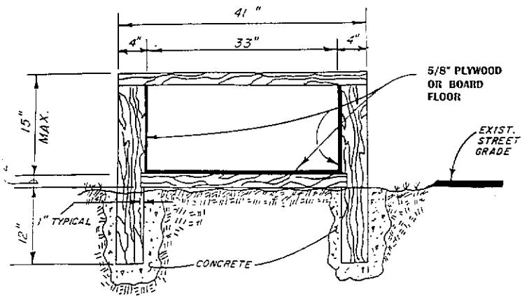
TYPICAL FRAMING PLAN
